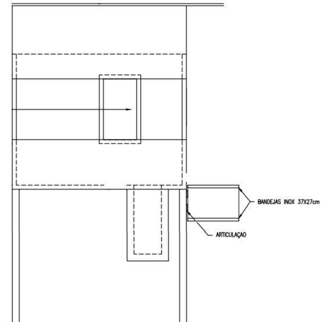
Vista frontal
